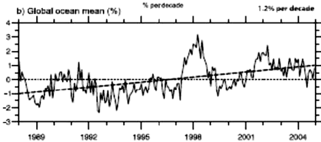
Figure 18. Plot of mean global monthly column water vapour anomalies since 1987 (from Figure 3.20 of page 372 of Solomon et al 2007), showing spurious “trend”
