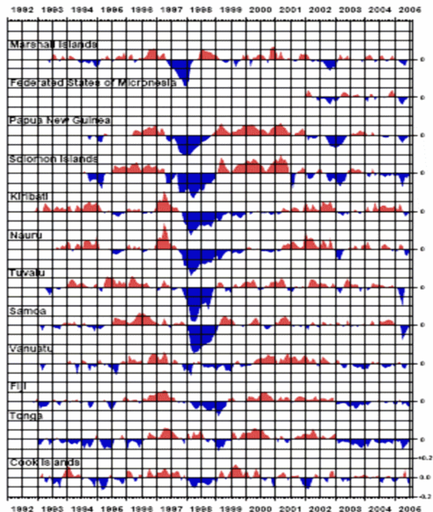
Figure 12. Sea Level records from 12 Pacific islands (Hall 2007)
