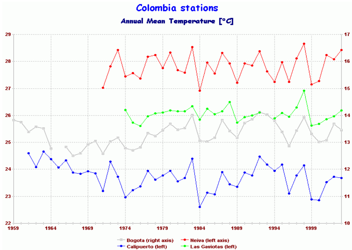
Figure 10. Temperature records from Colombia
