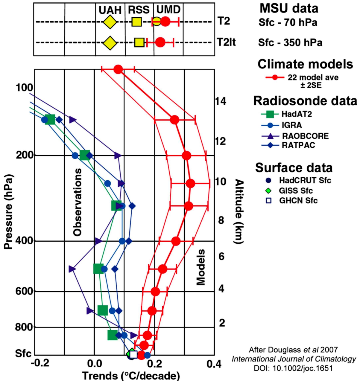
Figure 22. Comparison between model predictions and actual measurements of temperature change with height in the atmosphere (Douglass et al 2007)
