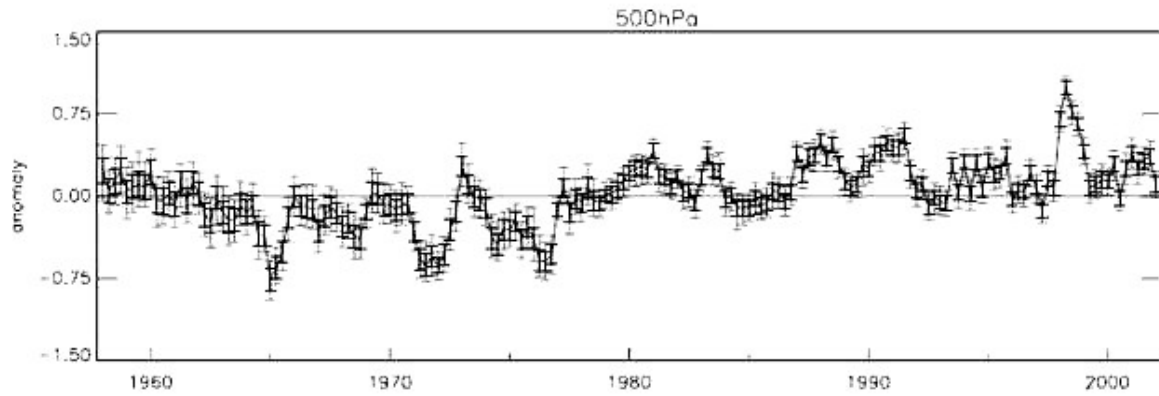
Figure 6. Global mean temperature record in the lower troposphere (500hPa) indicating 95% confidence levels (Thorne et al 2004)
