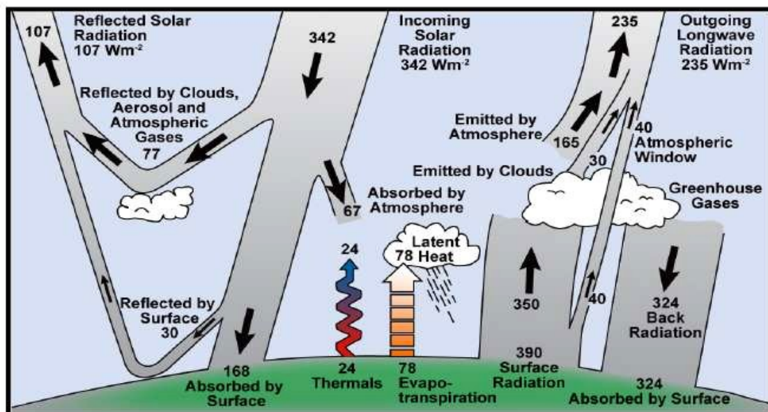
Figure 21. Earth's Annual Global Mean Energy Budget, as envisaged by Kiehl and Trenberth (1997) and published in “Climate Change 2007”
