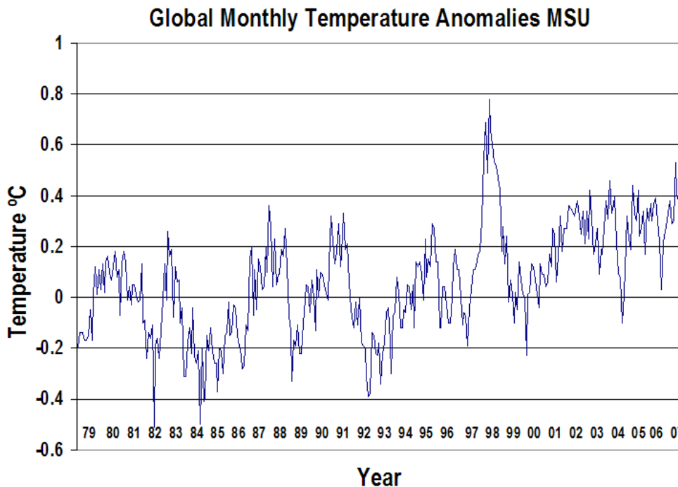
Figure 7. MSU (satellite) monthly global temperature anomaly record since 1979 for the lower troposphere (MSU 2007)
