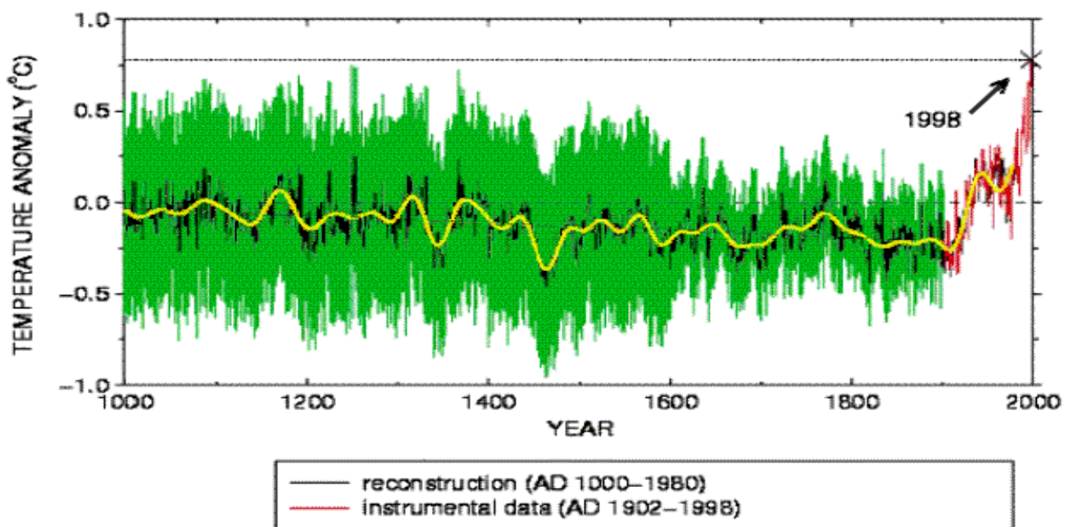
Figure 14. The "Hockey Stick" comparison for the Northern Hemisphere between past proxy temperature estimates and the recent Mean Annual Global Surface Temperature Record. (Houghton et al. 2001)
