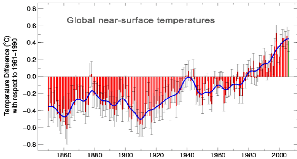
Figure 1. Mean Annual Global Surface Temperature Anomaly (Brohan et al 2006) showing 95% confidence levels
