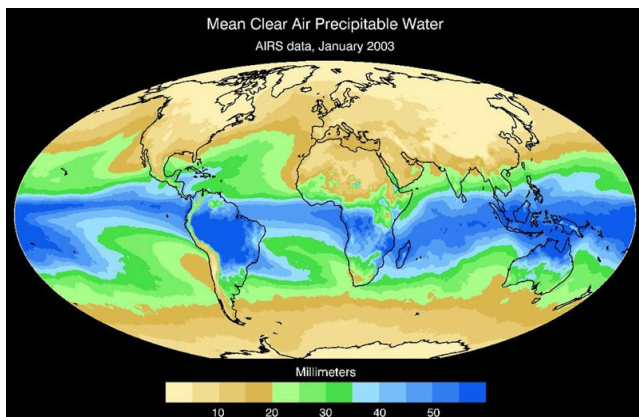
Figure 16. Total water vapour in the atmosphere for the month of January 2003, measured in mm. High value over 50mm, low to zero. (Encyclopaedia of Earth 2008)
