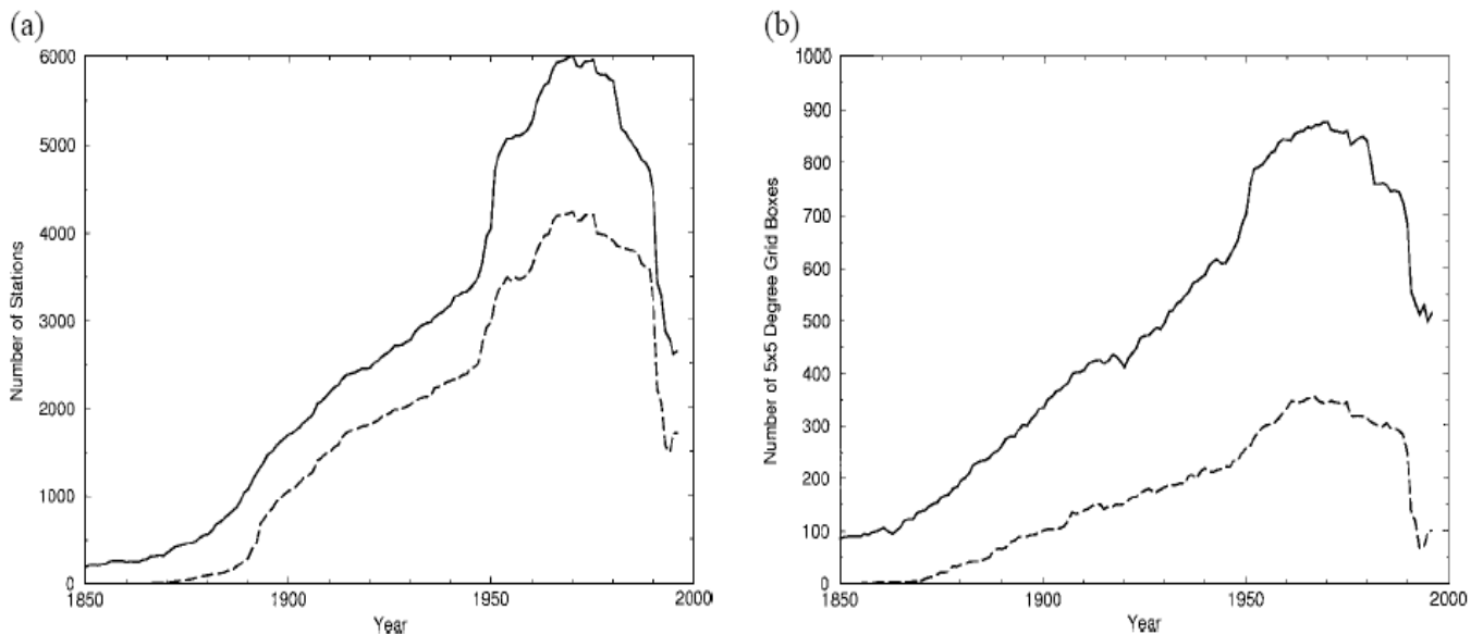
Figure 2. Number of available global weather stations for Northern and Southern Hemispheres, (a) and number of grid boxes available (b) from a theoretical total of 2,592 5°/5° latitude/longitude boxes (Hansen 2008)
