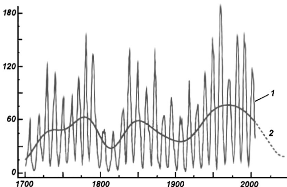
Figure 13. Record of Sunspot numbers (Abdussamatov 2005)
