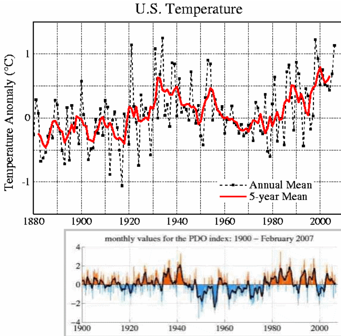
Figure 3. Corrected mean annual temperature anomaly record for the contiguous United States (Hansen 2008) compared with the Pacific Decadal Oscillation Index (Mantua 2007)
