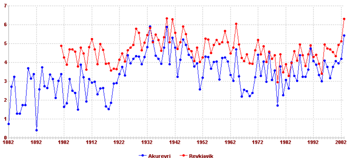
Figure 9. Temperature records for Reykjavik and Akureyri, Iceland
