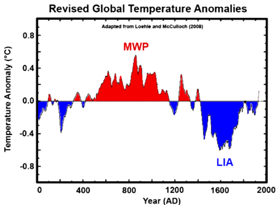
Figure 15. Proxy temperatures for the past 100 years ignoring tree rings (Loehle and McCulloch 2008)
