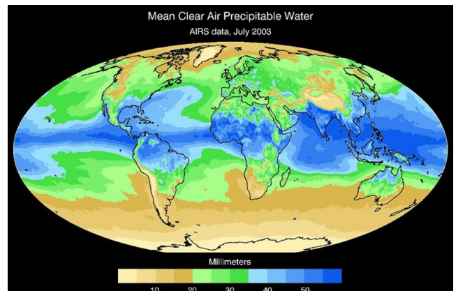
Figure 17. Total water vapour in the atmosphere for the month of July 2003, measured in mm. (Encyclopaedia of Earth 2008)
